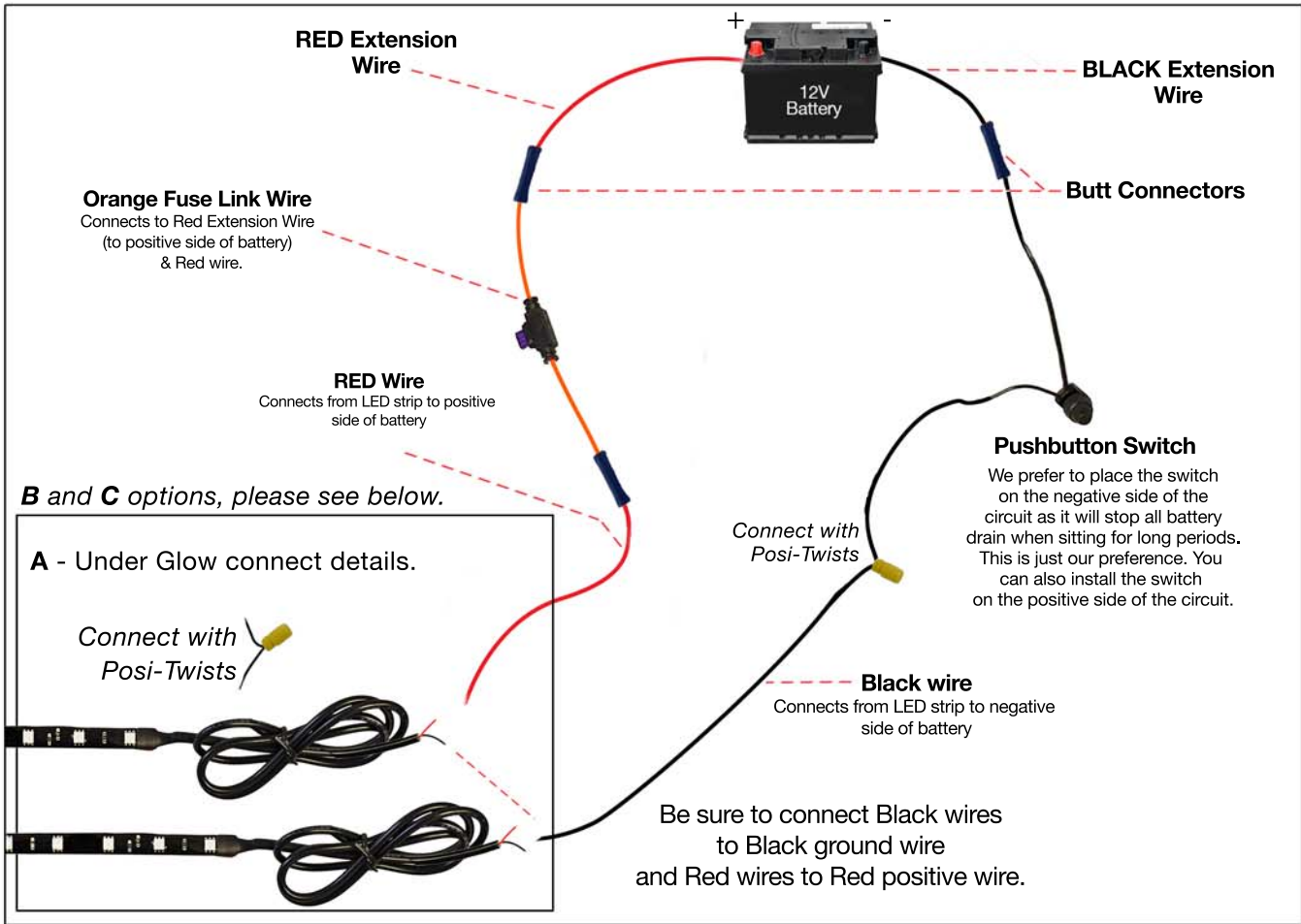
A - LED Strip Red & Black Wires. Connects w/ Red and Black Wires from Battery. Connect with a Posi-Twist. Red is the Positive wire, Black is the Ground wire.
