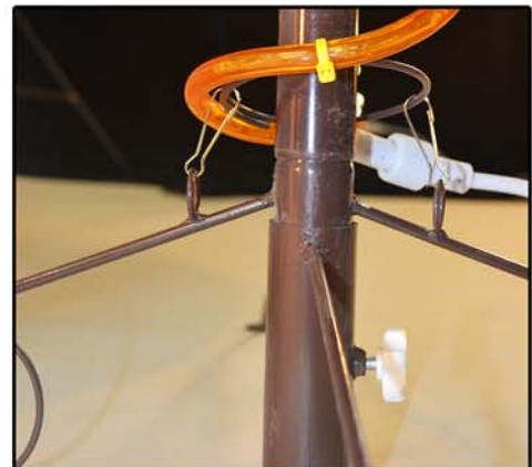
Tree bottom showing retaining clips and tree base lock.
